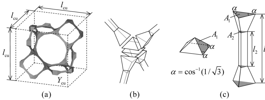
Figure 2: (a) Cubic unit cell Y_{cu} , (b) strut-junction connection, and (c) shape of struts and junctions
