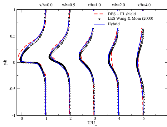
Figure 12. Velocity profiles at the wake
