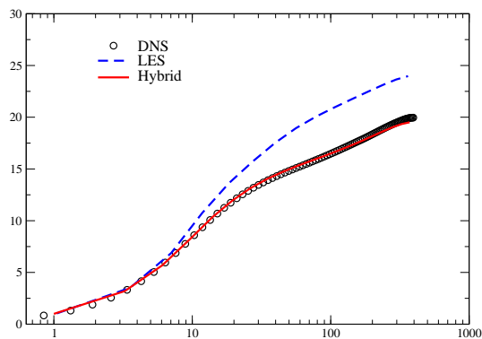
Figure 1. Velocity profile at Re_\tau = 395
