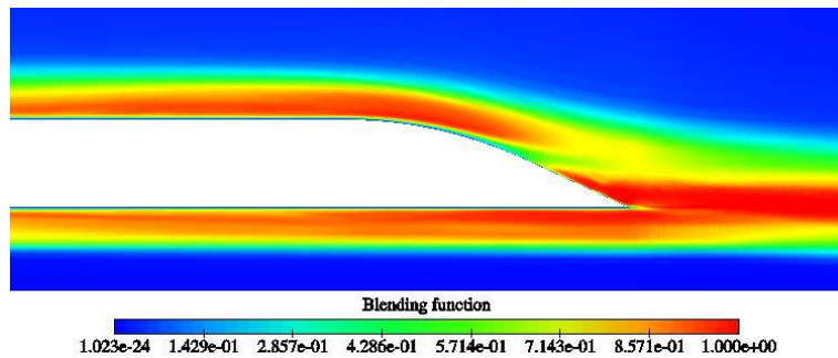
Figure 14. Blending function contours for the hybrid model
