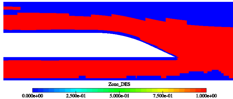
Figure 15. LES and RANS zones on DES simulation
