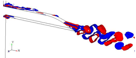
Figure 11. Iso-contours of u' , DES model
