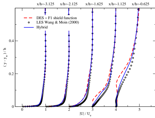
Figure 8. Velocity profiles over the aerofoil
