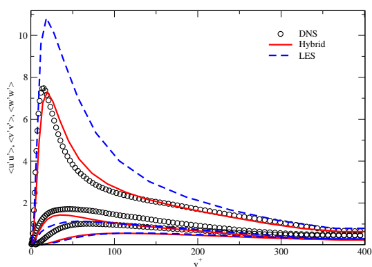
Figure 3. Normal stresses at Re_\tau = 395
