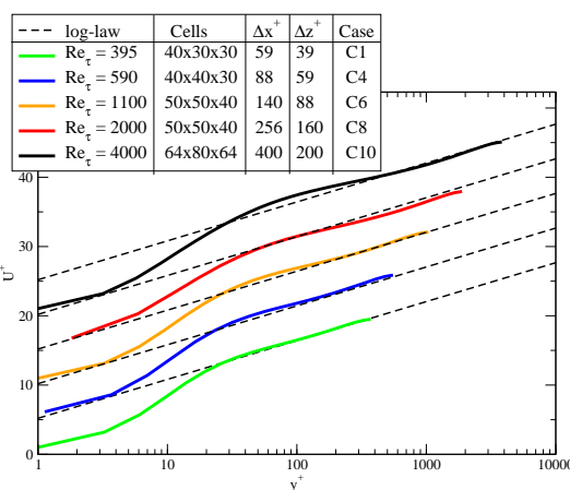
Figure 4. Velocity profiles at different Reynolds numbers.
