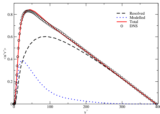
Figure 2. Shear stress at Re_\tau = 395
