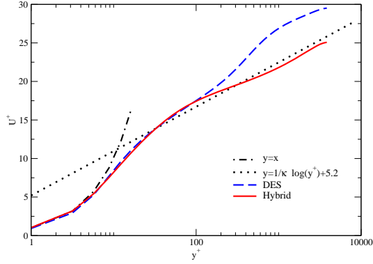
Figure 5. Velocity profiles at Re_\tau = 4000
