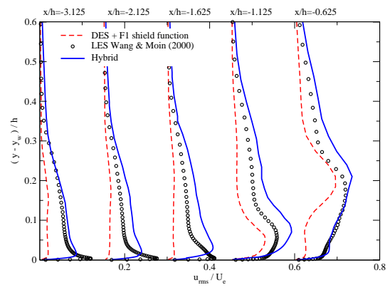
Figure 9. u_{rms} profiles over the aerofoil
