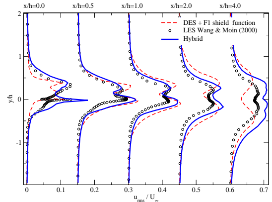
Figure 13. u_{rms} profiles at the wake
