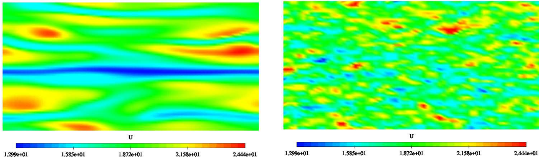
Figure 6. Instantaneous streamwise velocity contours. DES
