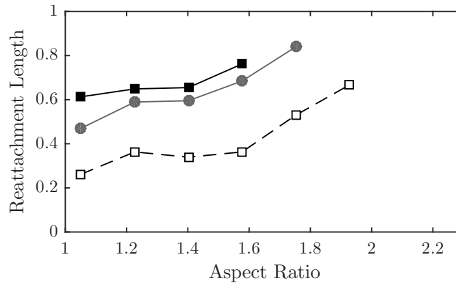
FIGURE 6.8: Reattachment length of time-averaged flow along the slant. Symmetry plane y/W = 0 (—■—), y/W = 1/6 (—●—) and y/W = 1/3 (-□-).
