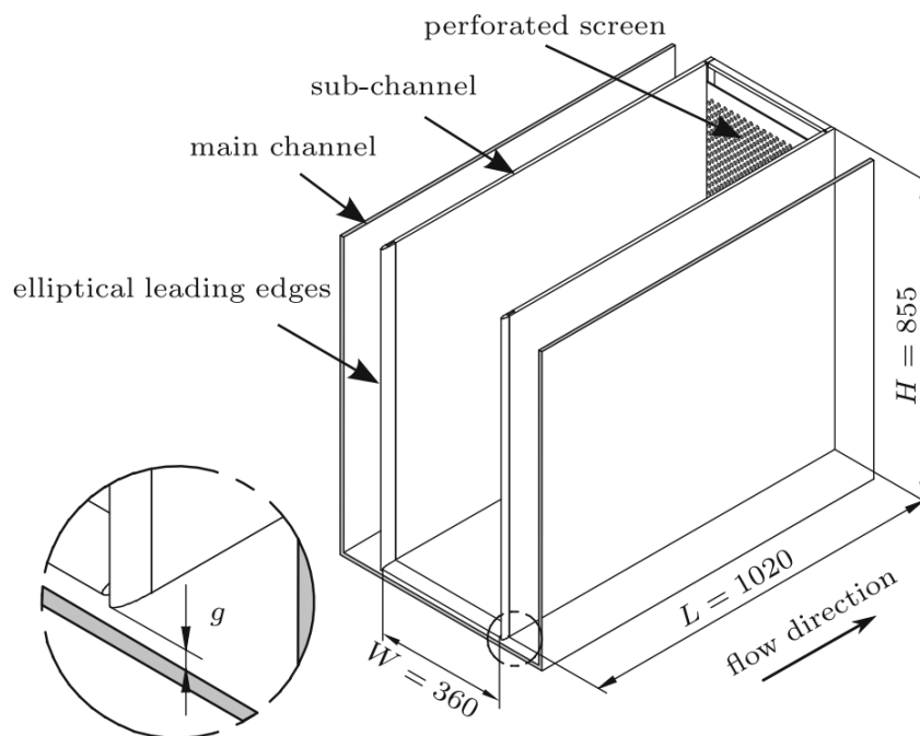
FIGURE 3.3: Geometry of the sub-channel flow velocity reduction device. Radi et al. (2014)
