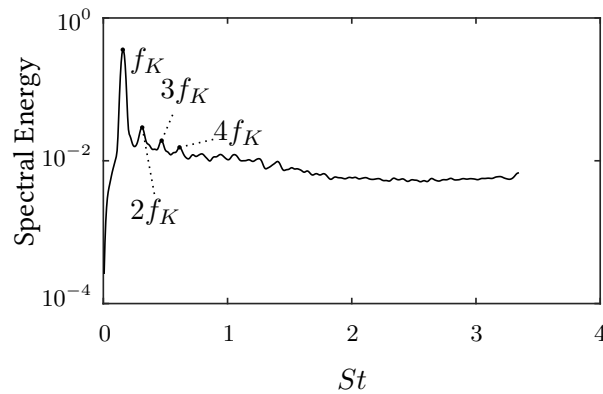
FIGURE 4.35: Spectral energy behind the trailing-edge of the flat plate at 50^\circ .
