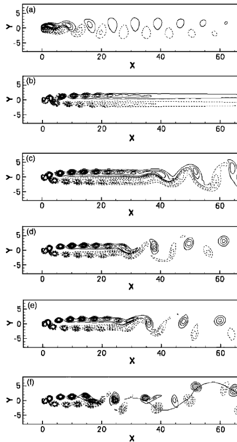
FIGURE 2.36: Instantaneous spanwise vorticity contours showing the effect of Reynolds number on the far wake. (a) Re = 35 ; (b) Re = 100 ; (c) Re = 145 ; (d) Re = 150 ; (e) Re = 150 ; (f) Re = 175 . From Saha (2007).
