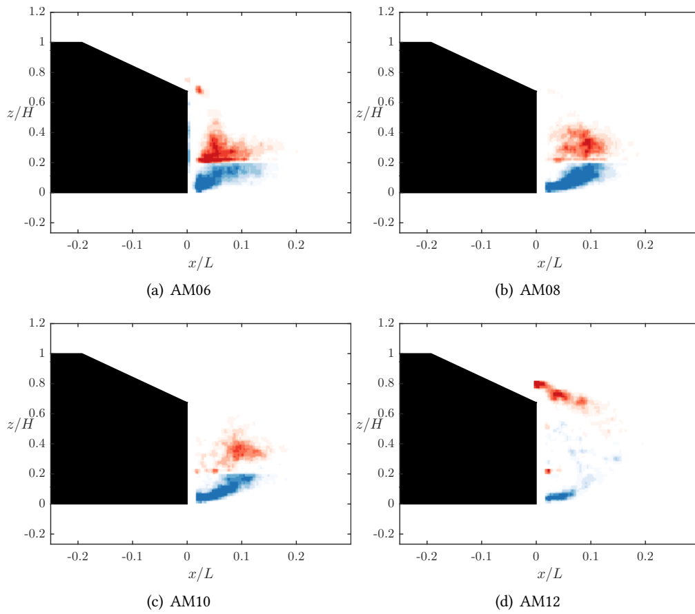
FIGURE 6.22: Distribution of the maximum (red) and minimum (blue) of the \Gamma_1 field, highlighting the variation of the cores of the A and B vortices respectively. Time-resolved data at y/W = \frac{1}{3} .
