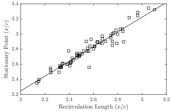
FIGURE 4.20: Correlation between the measured recirculation length ( RL ) and the location of the stationary eigenmode ( SP ). Linear fit is SP = 0.976 \times RL + .295 .
