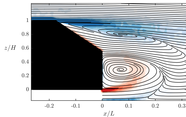
(b) C_D = 0.45
