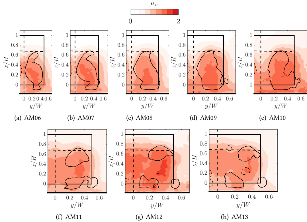
FIGURE 6.29: Standard deviation of v velocity component in the wake at downstream position x/L = 0.4 . Black contours represent time-averaged vortex bounds with dashes indicating negative rotation.
