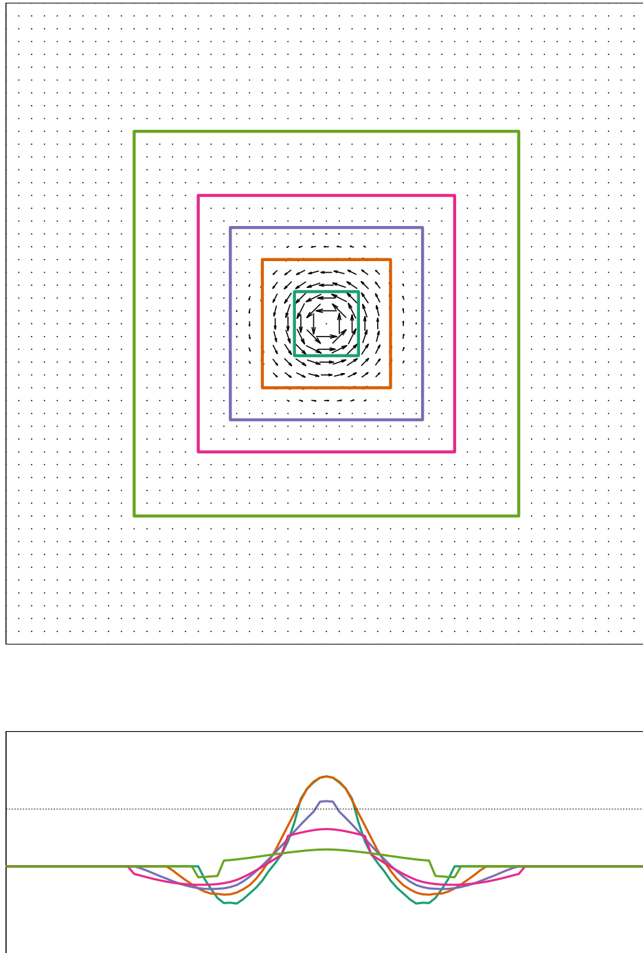
FIGURE 3.26: Comparison of \Gamma_2 calculations with changing region sizes. The various interrogation window sizes are denoted by the various colours. The \Gamma_2 strength as varies across the x -dimension is plotted below.
