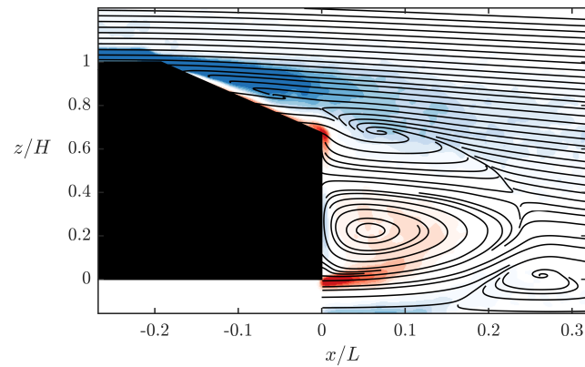
(a) C_D = 0.61
