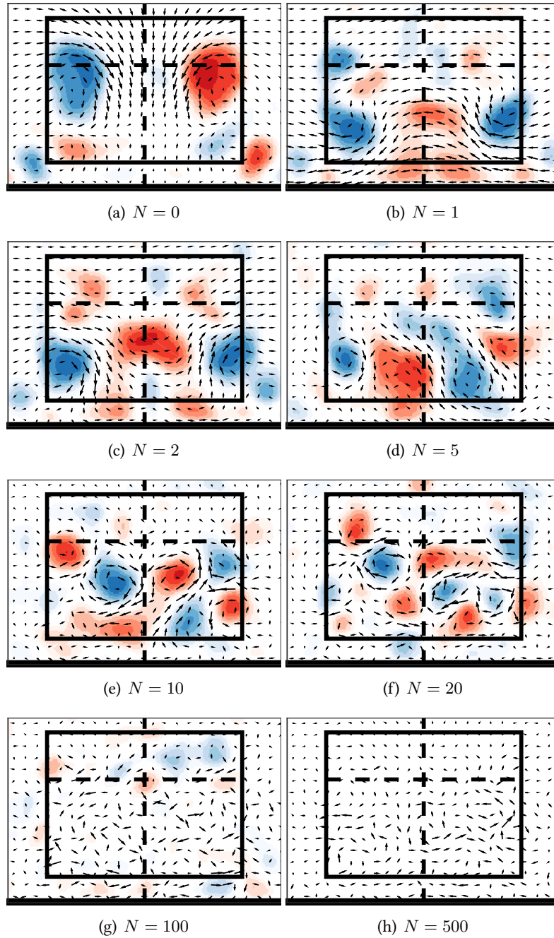
FIGURE 3.31: The spatial POD modes in the wake of the Ahmed body. The modes are represented by the vector field, with the filled contours representing the rotation in that field.
