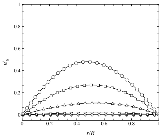
Figure 6: The relative azimuthal velocity along the free surface for different Rayleigh numbers at (a) Re = 10 and (b) Re = 1000 .
