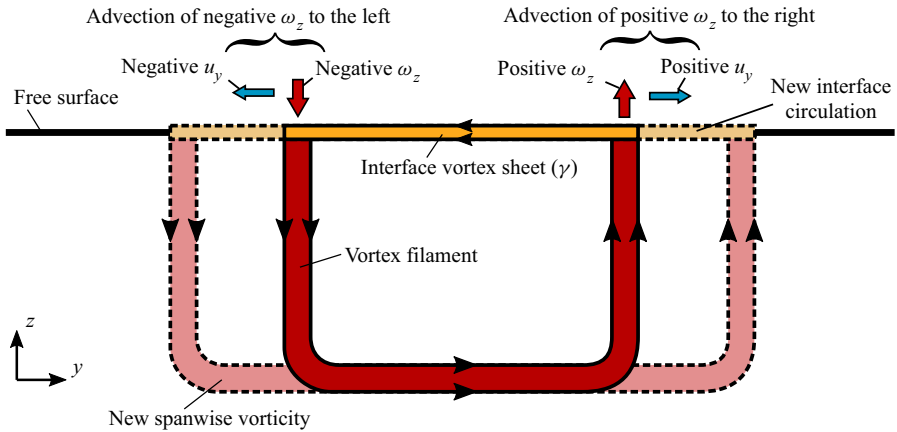
Figure 18. Illustration of the vortex stretching/tilting flux \mathbf{u}(\boldsymbol{\omega} \cdot \hat{\boldsymbol{s}}) from (4.6). This term can be interpreted as representing the advection of vortex filaments in the free surface, which must correspond to the creation of spanwise vorticity by vortex stretching in the fluid interior. An equal and opposite quantity of circulation is also created in the interface vortex sheet, so that the total spanwise circulation is conserved.
