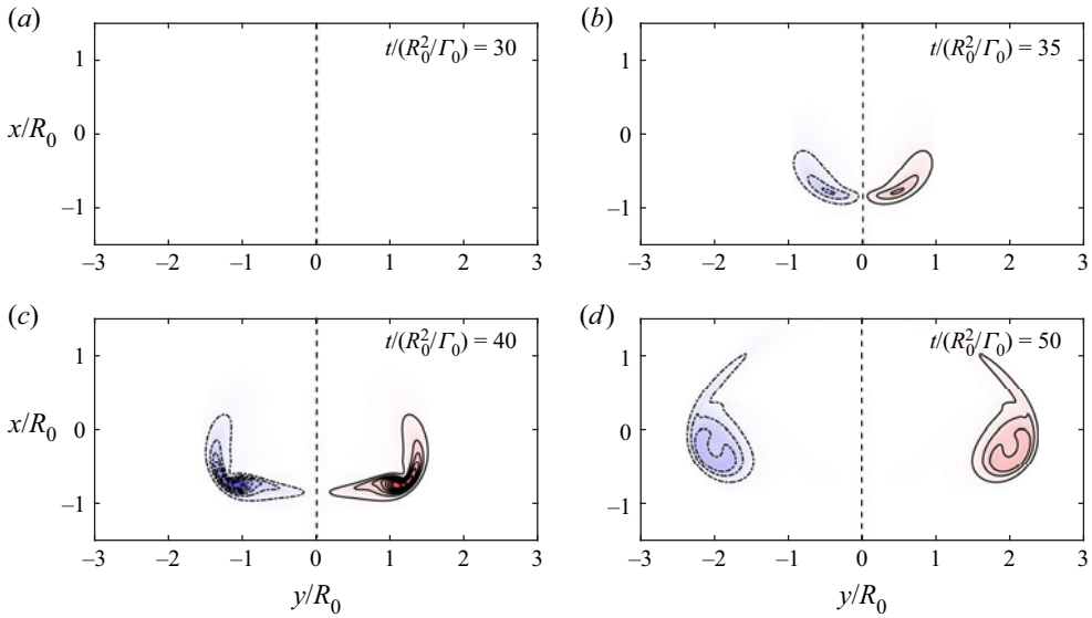
Figure 23. Contours of surface-normal vorticity ( \boldsymbol{\omega} \cdot \hat{\boldsymbol{s}} ) in the free surface at several times throughout the interaction. The colourmap and contour levels are the same as in figure 19. The dashed line indicates the connection line ( y = 0 ), which is the shared boundary of the surfaces I_1 , I_2 and S_1 .
