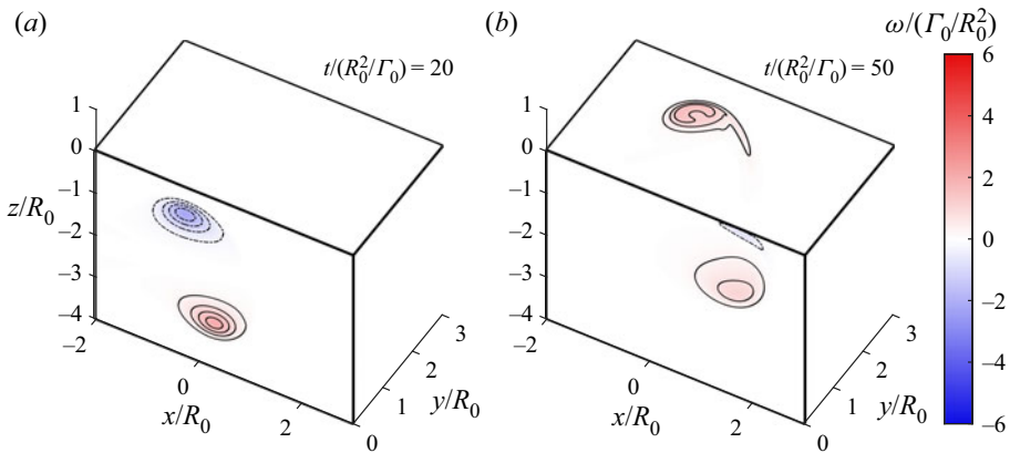
Figure 19. Contours of spanwise vorticity ( \omega_y ) in the symmetry plane ( y = 0 ), and of surface-normal vorticity ( \boldsymbol{\omega} \cdot \hat{\boldsymbol{s}} ) in the free surface, both (a) before and (b) after the free surface connection has occurred. Contours of dimensionless vorticity are plotted for \omega/(\Gamma_0/R_0^2) = \dots, -1.25, -0.75, -0.25, 0.25, 0.75, 1.25, \dots
