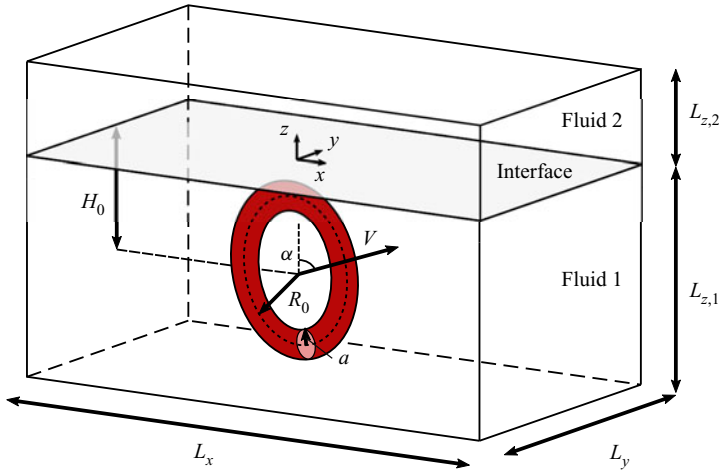
Figure 1. Flow configuration considered in this study. A vortex ring of circulation \Gamma_0 , radius R_0 and core radius a is positioned at depth H beneath the interface (or free surface), and approaches the interface at angle \alpha . The computational domain is a box with side lengths L_x , L_y , and L_{z,1} (in fluid 1) and L_{z,2} (in fluid 2). For free-surface flows, the upper fluid is ignored, and the interface is replaced with the free-surface boundary.
